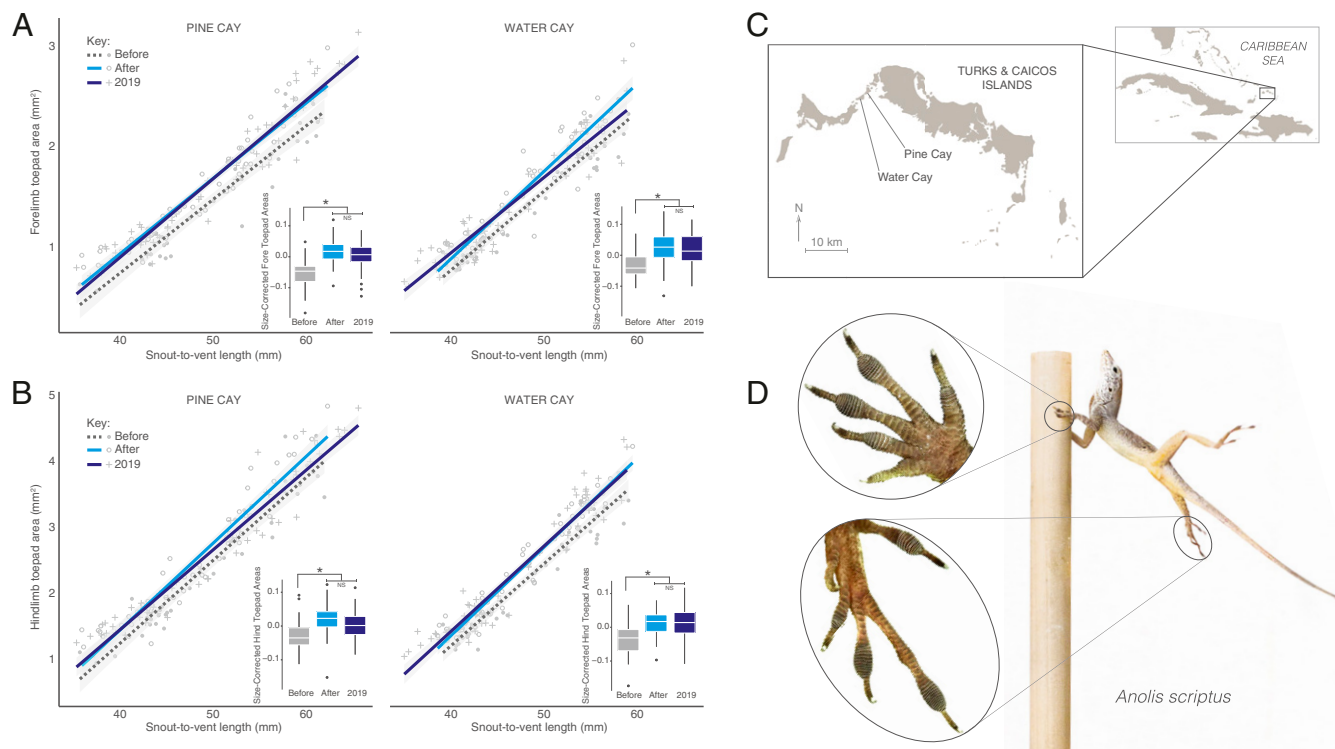
Fig. 1. Anolis scriptus , like other anoles, use specialized toepads to cling to surfaces ( D , Inset images: A lizard clings to a perch while experiencing hurricane-force winds in a performance experiment; see ref. 3). Populations of A. scriptus on Pine and Water Cays in the TCI ( C ) that survived 2017's Hurricanes Irma and Maria had relatively larger toepads on average than the populations surveyed before the storms (3). When we resurveyed the populations in 2019 ( A and B ) following the storms, those body size-corrected differences in toepad area persisted.
